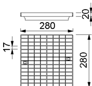
Galvanized mesh grating 20/30, B 125
