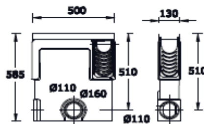
Silt box MEADRAIN Z/S 1000.EK
